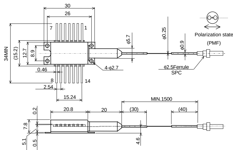
Package outline(Unit:mm) Type:AF4A1224A75L
